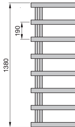
Front view ALZ-140-050
