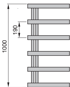
Front view ALZ-100-050
