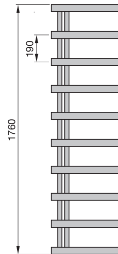
Front view ALZ-180-050
