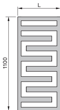
Front view TET-110-050
